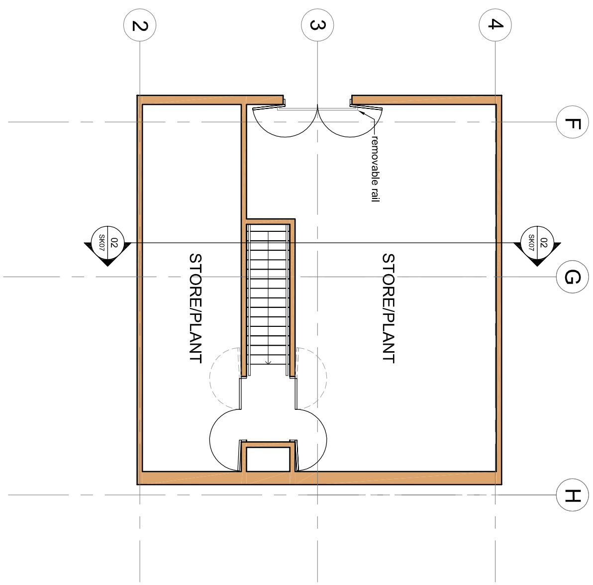
1. PROPOSED FIRST FLOOR PLAN 1:100@A3
